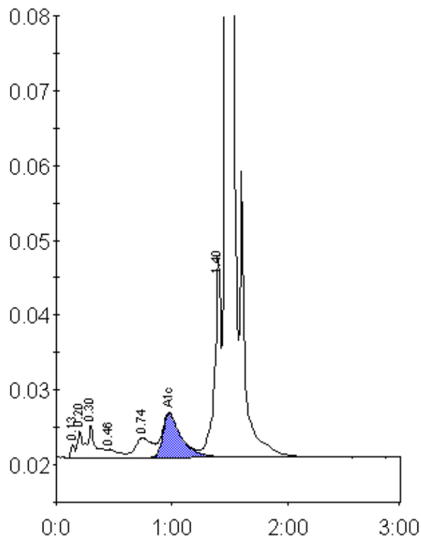
Peak table - ID: 10498302
